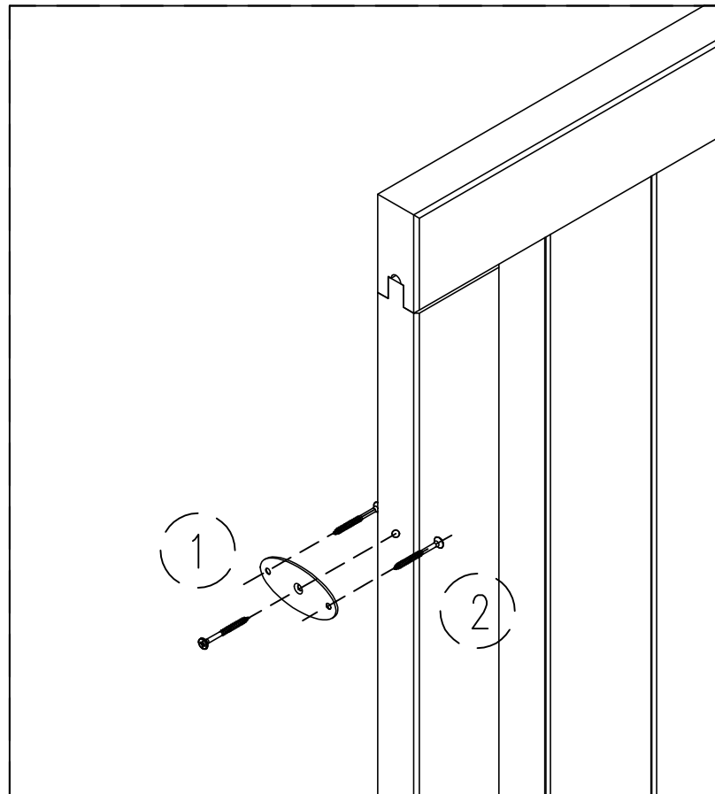
F (1:5)
