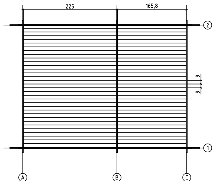
FLOOR BOARDS - FUSSBODENBRETT - PLAN POSE PLANCHER
