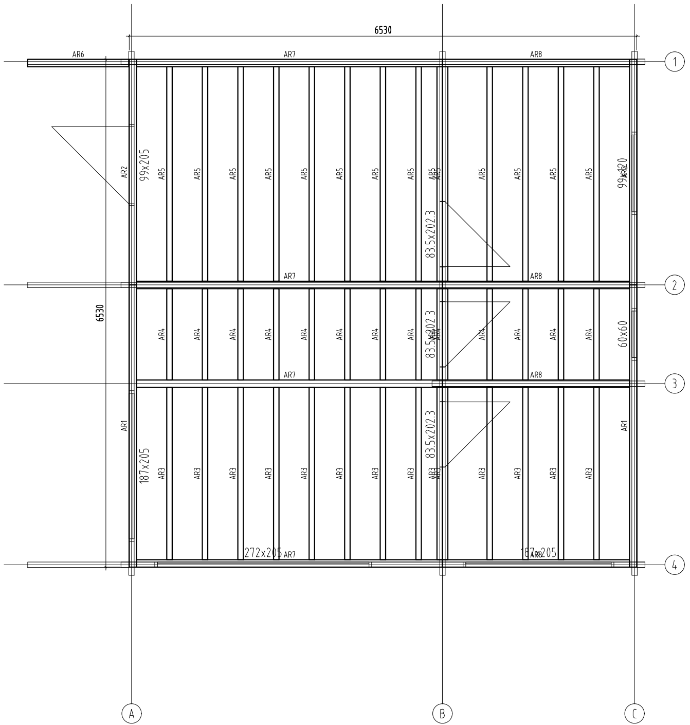
Foundation plan
