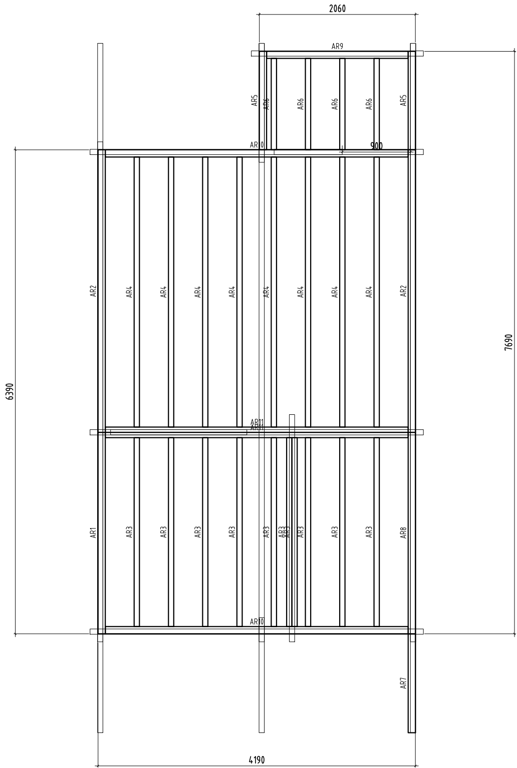
Foundation plan
